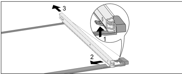
Fig. 117 Glass shelf with rails
