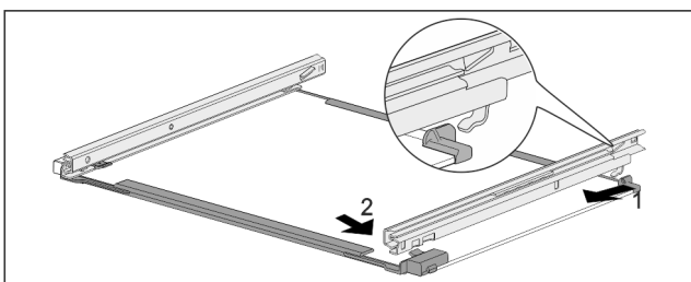
Fig. 119 Glass shelf with rails
