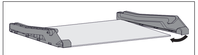
Fig. 29 Glass shelf with side parts
