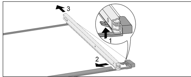
Fig. 109 Glass shelf with rails
